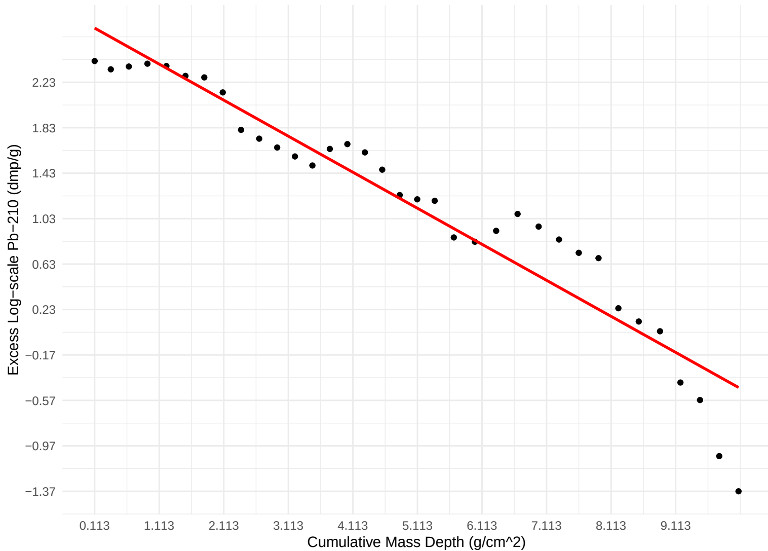
Excess Log-scale Pb-210 vs Mass Depth
